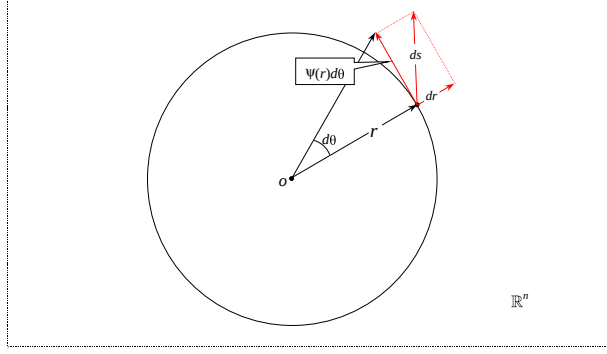
Figure 1: The Riemannian metric on a model manifold
