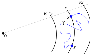
Figure 5: Path \gamma connects points x and y in B(o, Kr) \setminus B(o, K^{-1}r)
