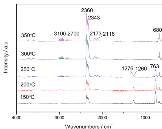
Fig. 2 On-line IR spectra of DCM conversion over V-Ni/TiO 2 catalyst with the increased reaction temperature.
