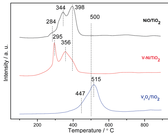
Fig. 5 H 2 -TPR profiles of as-prepared catalysts.
