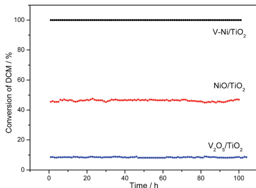
Fig. 9 Stability test of catalysts in DCM conversion at 300 °C; gas composition: 1000 ppm DCM, 20.8% O 2 , N 2 balance, GHSV = 15 000 mL g -1 h -1 .
