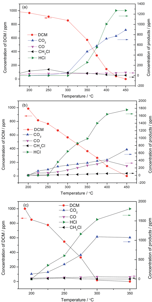
Fig. 3 DCM conversion and the products distribution: (a) V 2 O 5 /TiO 2 ; (b) NiO/TiO 2 ; (c) V-Ni/TiO 2 . Gas composition: 1000 ppm DCM in air, GHSV = 15 000 mL g -1 h -1 .
