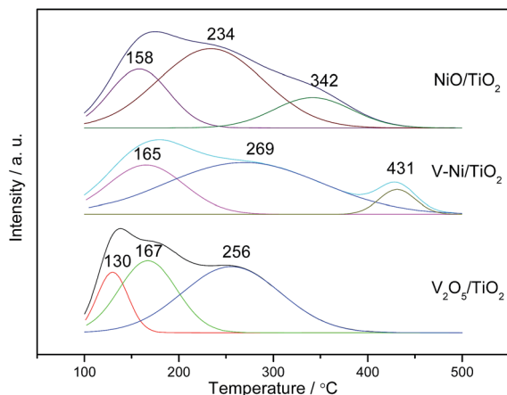
Fig. 6 \text{NH}_3 -TPD profiles of investigated samples.
