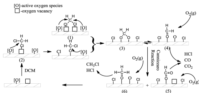
Fig. 11 A plausible mechanism for DCM combustion over V-Ni/TiO 2 .
