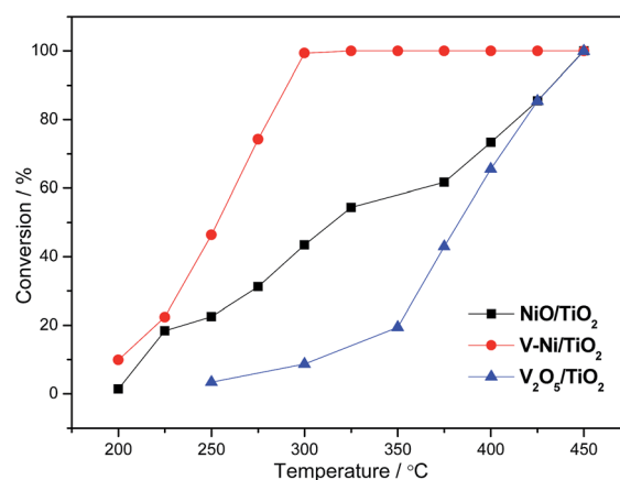
Fig. 1 Light-off curves of DCM over as-prepared catalysts. Gas composition: 1000 ppm DCM in air, GHSV = 15\,000 \text{ mL g}^{-1} \text{ h}^{-1} .
