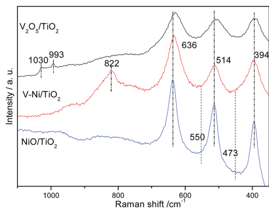
Fig. 7 Raman patterns of investigated samples.
